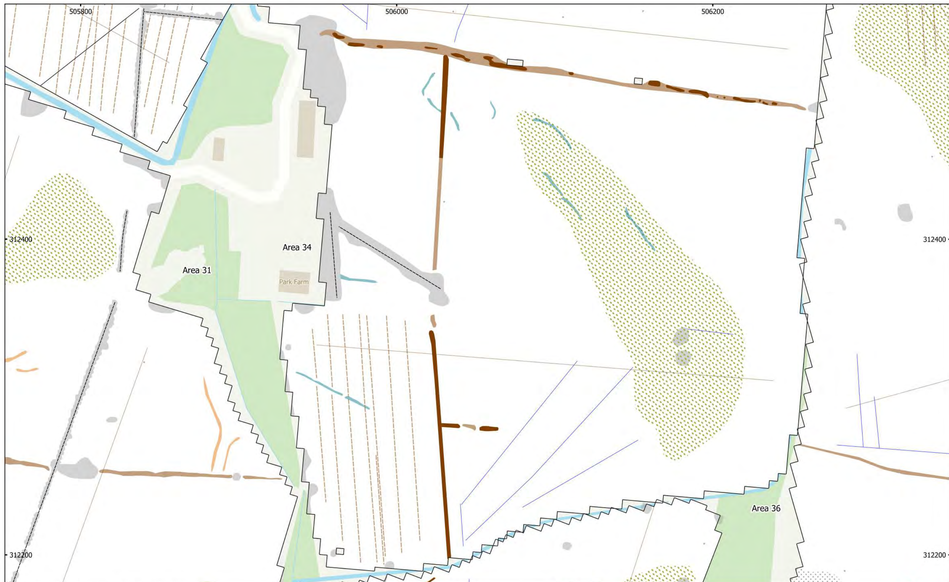
MSTF1136: Mallard Pass, DCO, Essendine, Rutland Figure 106 - Magnetic Interpretation (Areas 31, 34 & 36) 1:1,500 @ A3
